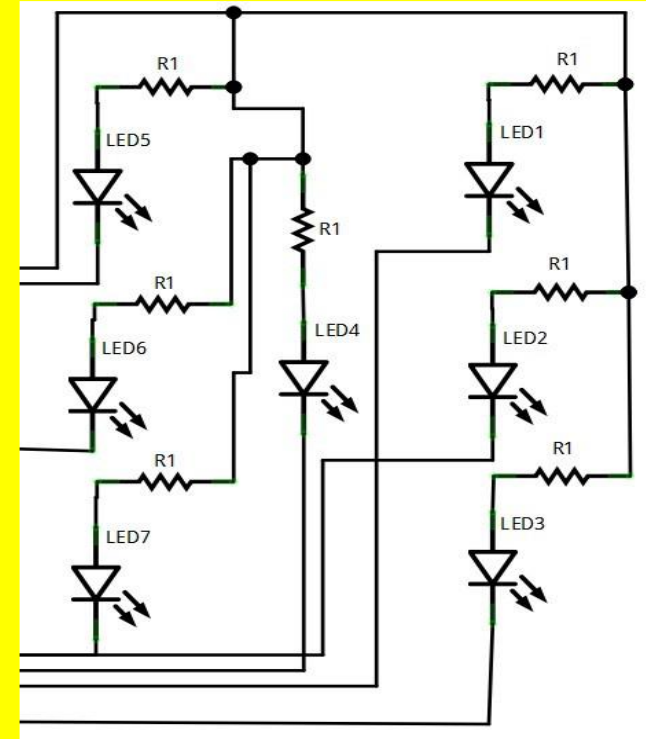
Figure 1.3.2 : Schematic Diagram For LED Dice
