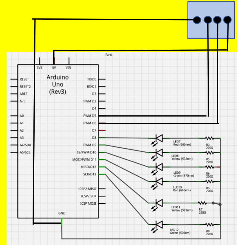
Figure 2.1.1 : Hardware Connection For Obstacle Sensor Using Aduino And HCSR04
