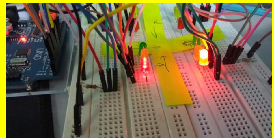
Figure 1.8.2 : OutputFor Traffic Signal Model (Automatic 3 Traffic Light)
