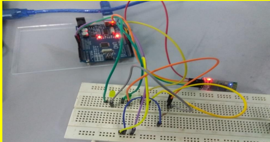
Figure 2.6.2 : Hardware Connection For Aduino HC-06 Serial Port Bluetooth Module
