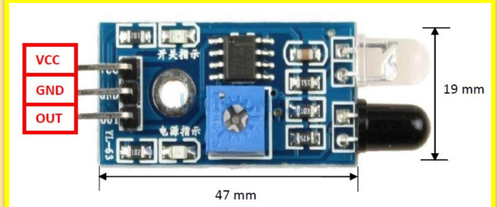
Figure 2.3.1 : Hardware Connection For Infrared Barrier Module
