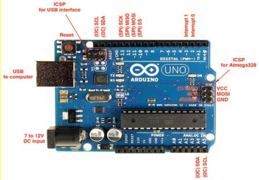
Figure 1.1 : Adruino Uno open-source microcontroller board
