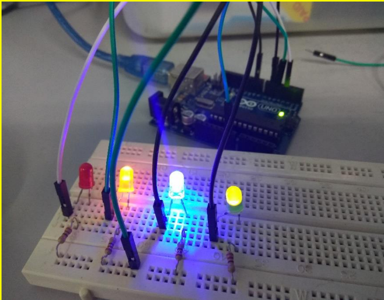
Figure 3.15.2 : Timer Output
