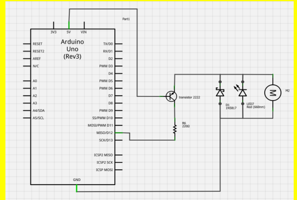
Figure 2.4.1 : Hardware Connection For Aduino Infrared Collision Avoidance & Motor
