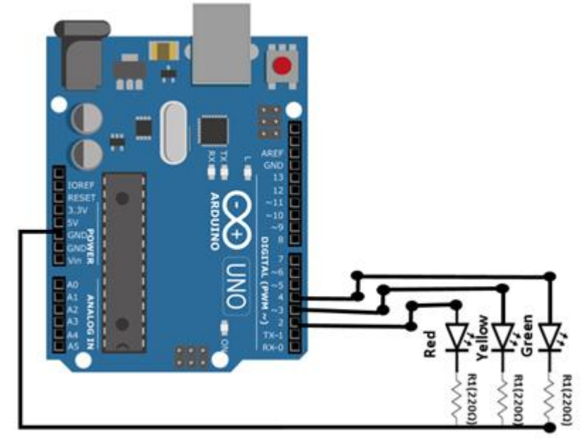
Figure 1.6.1 : Hardware Connection For Traffic Signal Model (Automatic)
