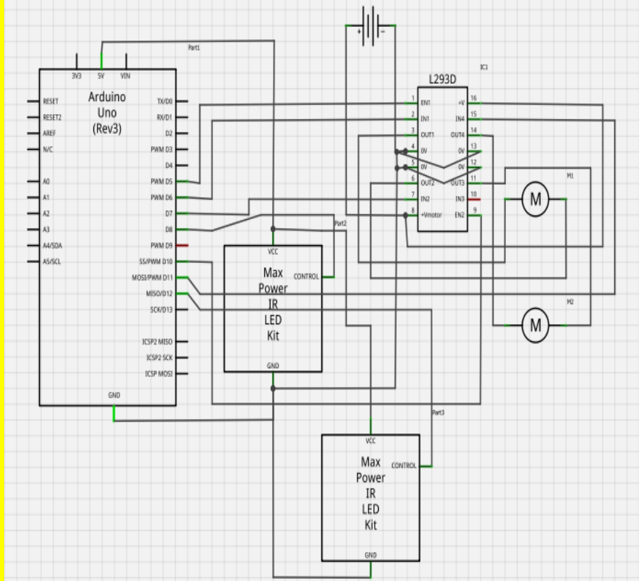
Figure 2.7.1 : Hardware Connection For Adruino L293D DC motors control (2 Motor)
