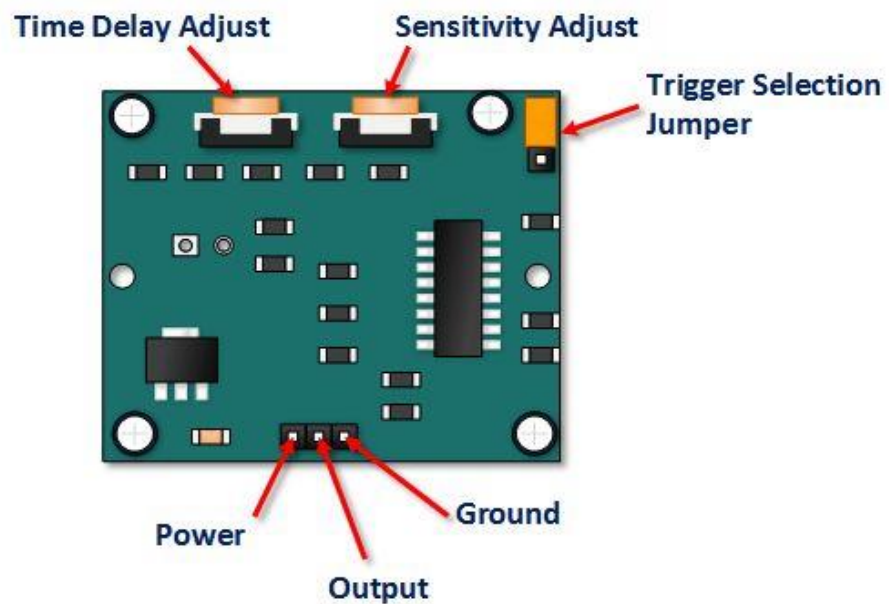
Figure 3.22.12 : Motion Detector Board
