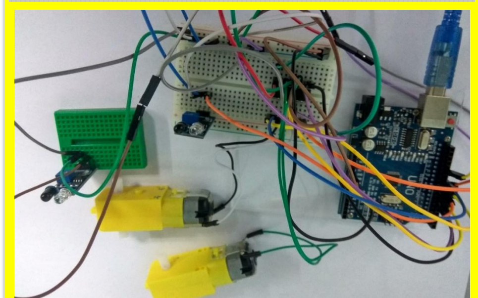
Figure 2.7.2 : Output For Adruino L293D DC motors control (2 Motor)
