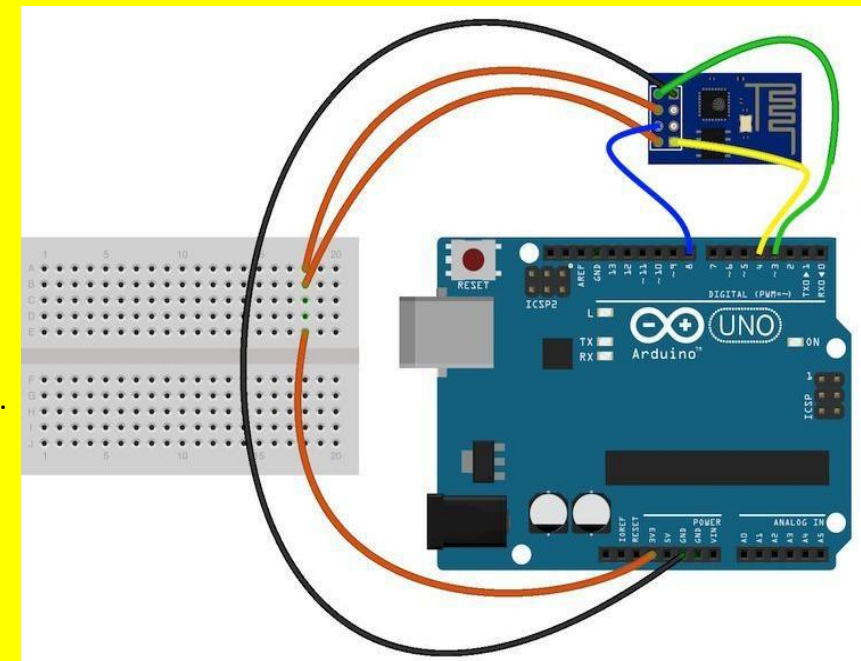
Figure 3.10.4 : Hardware Connection For ESP8266
