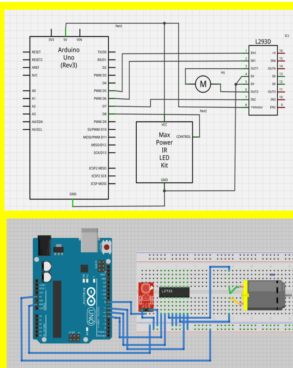
Figure 2.5.1 : Hardware Connection For Aduino L293D DC motors control
