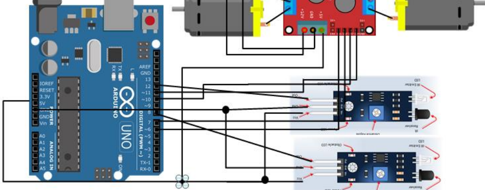
Figure 2.8.1 : Hardware Connection For Adruino L298D ROBOT CAR
