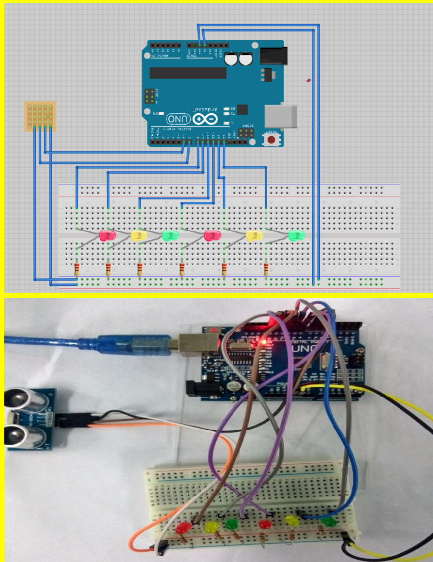
Figure 2.1.2 : Output For Obstacle Sensor Using Adruino And HCSR04
