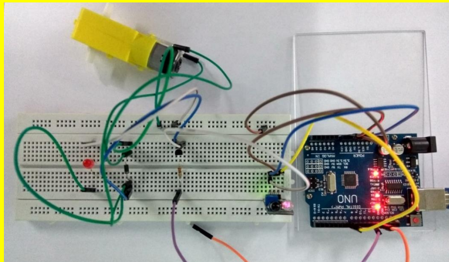
Figure 2.4.2 : Output For Arduino Infrared Collision Avoidance & Motor
